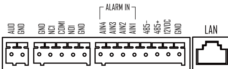
Figure 2-6 Alarm Input Device Wiring
