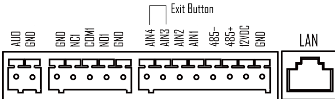
Figure 2-5 Exit Button Wiring
