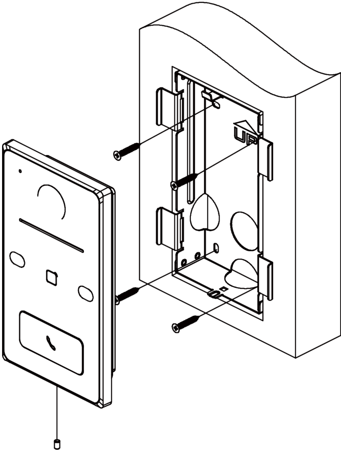
Figure 3-3 Flush Mounting
