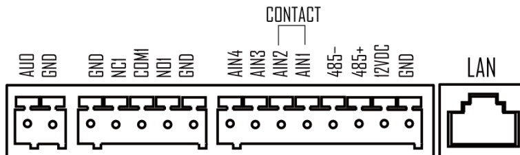
Figure 2-4 Door Contact Wiring
