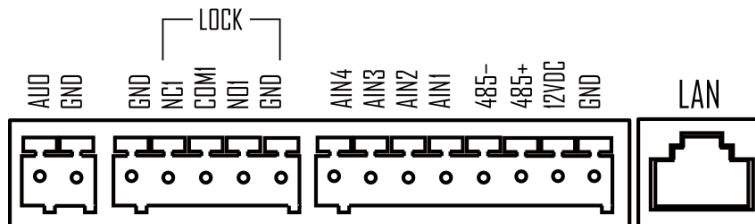
Figure 2-3 Door Lock Wiring
