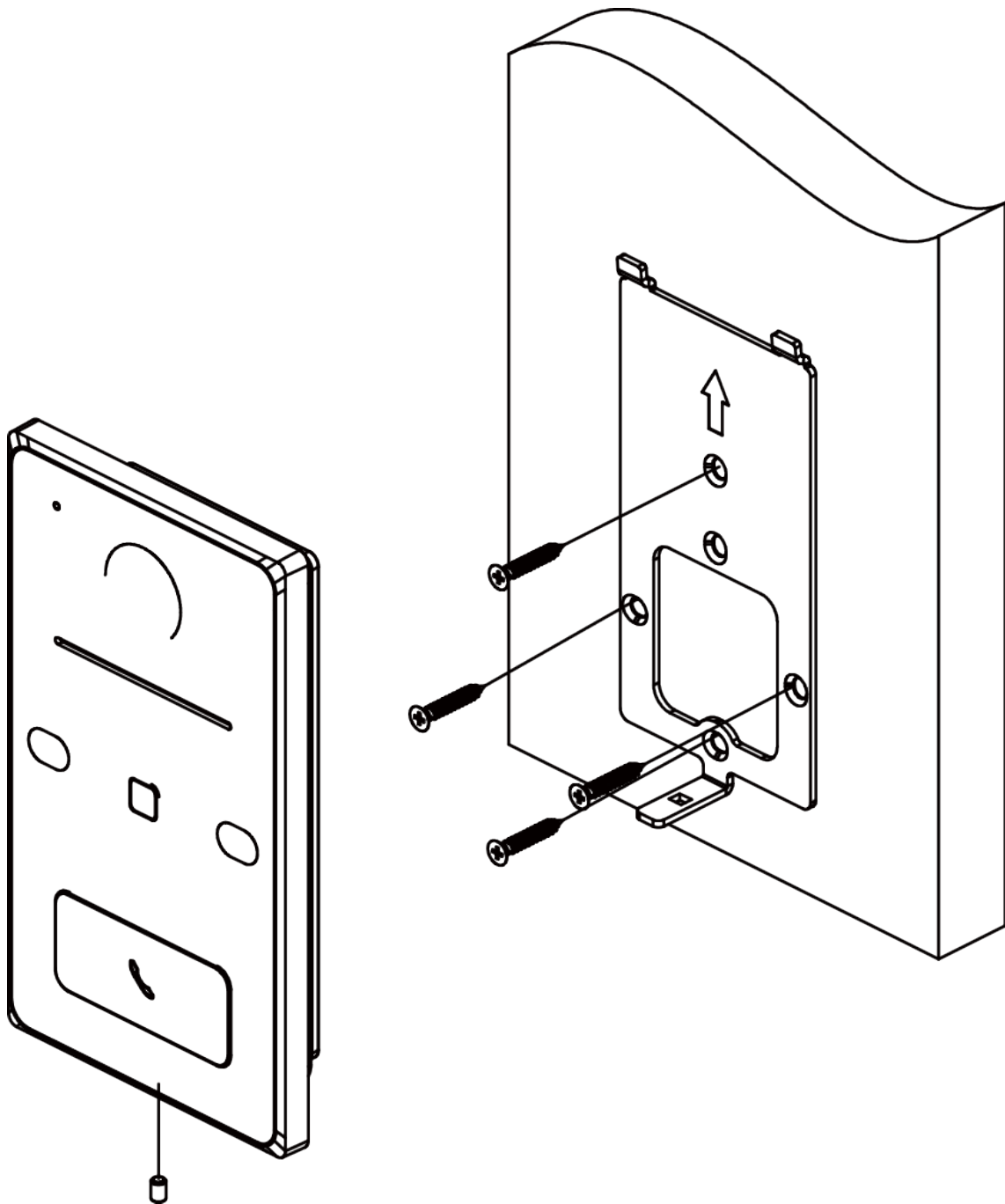
Figure 3-2 Surface Mounting
