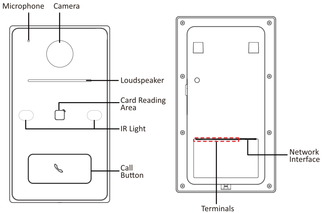
Figure 1-1 Front Panel and Rear Panel
