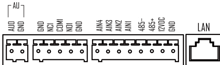
Figure 2-2 Audio Output Wiring
