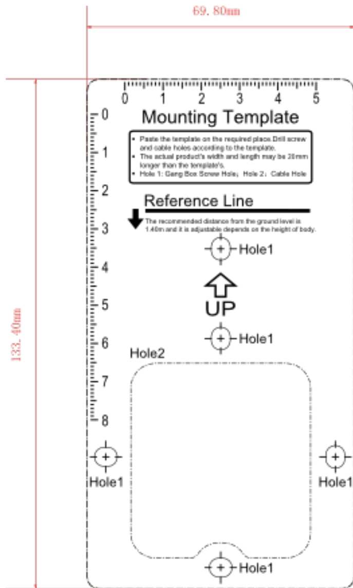
Figure 3-1 Mounting Template
